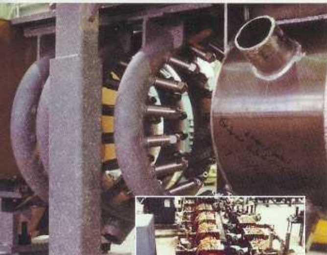
Seamless and ERW pipe and casing is hardened and tempered at production rates up to 120 tons per hour.
